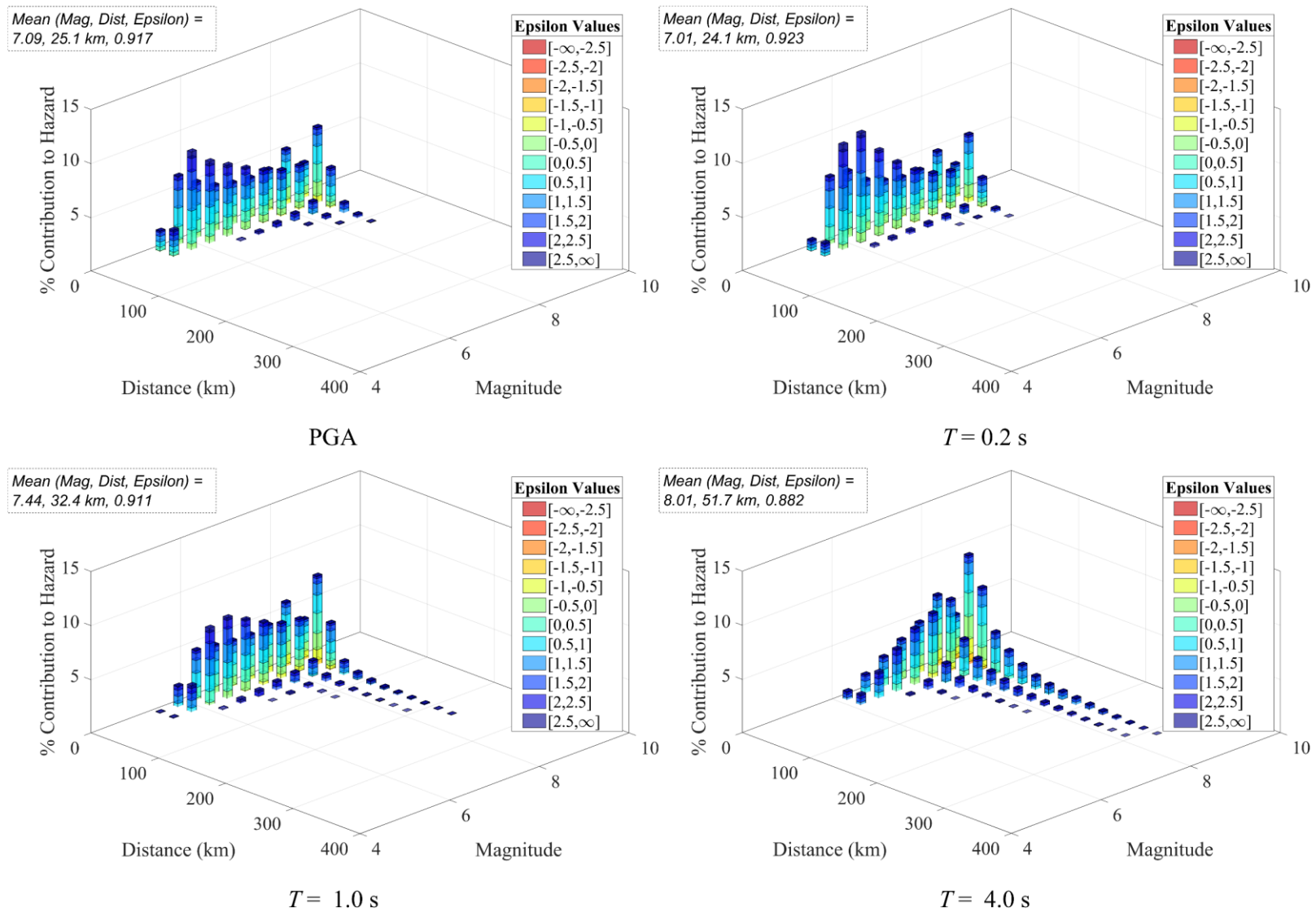
Fig. S2. Disaggregation of the hazard at the Dehradun site for 1500-year return period.
