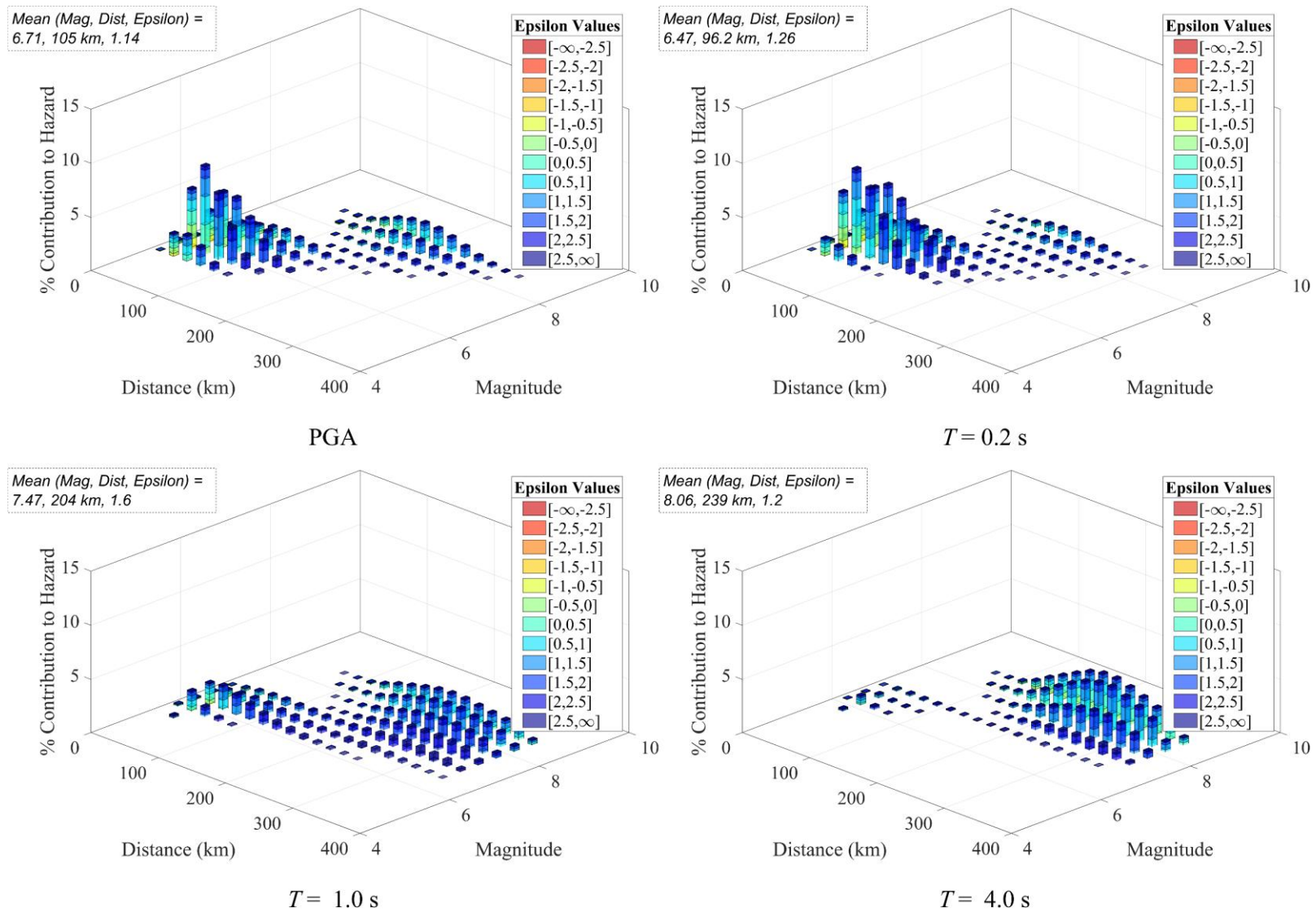
Fig. S6. Disaggregation of the hazard at the New Delhi site for 1000-year return period.
