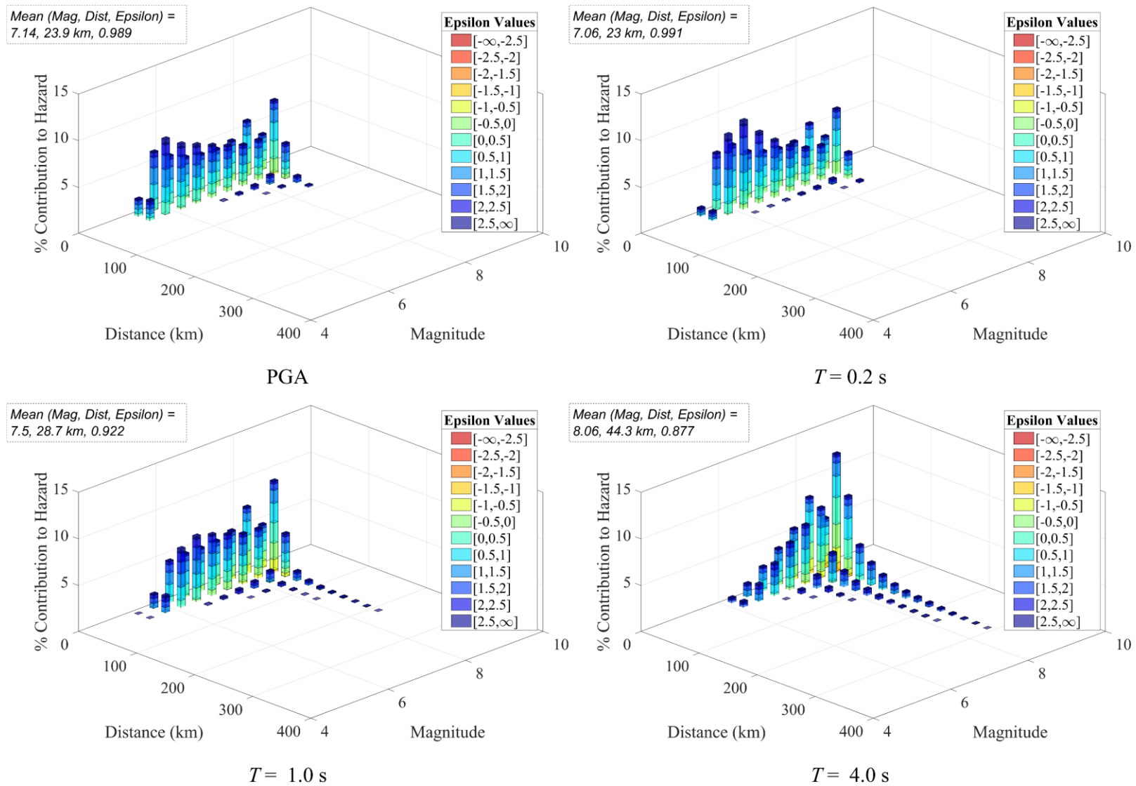
Fig. S3. Disaggregation of the hazard at the Dehradun site for 2000-year return period.
