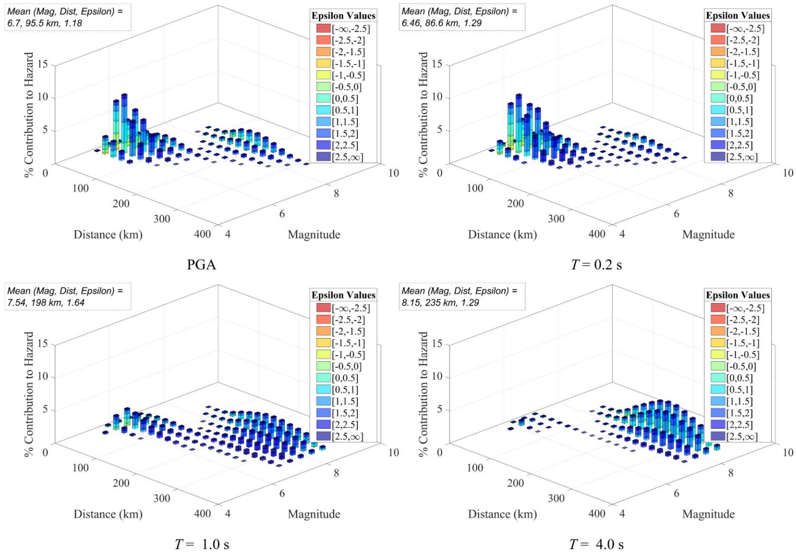
Fig. S7. Disaggregation of the hazard at the New Delhi site for 1500-year return period.
