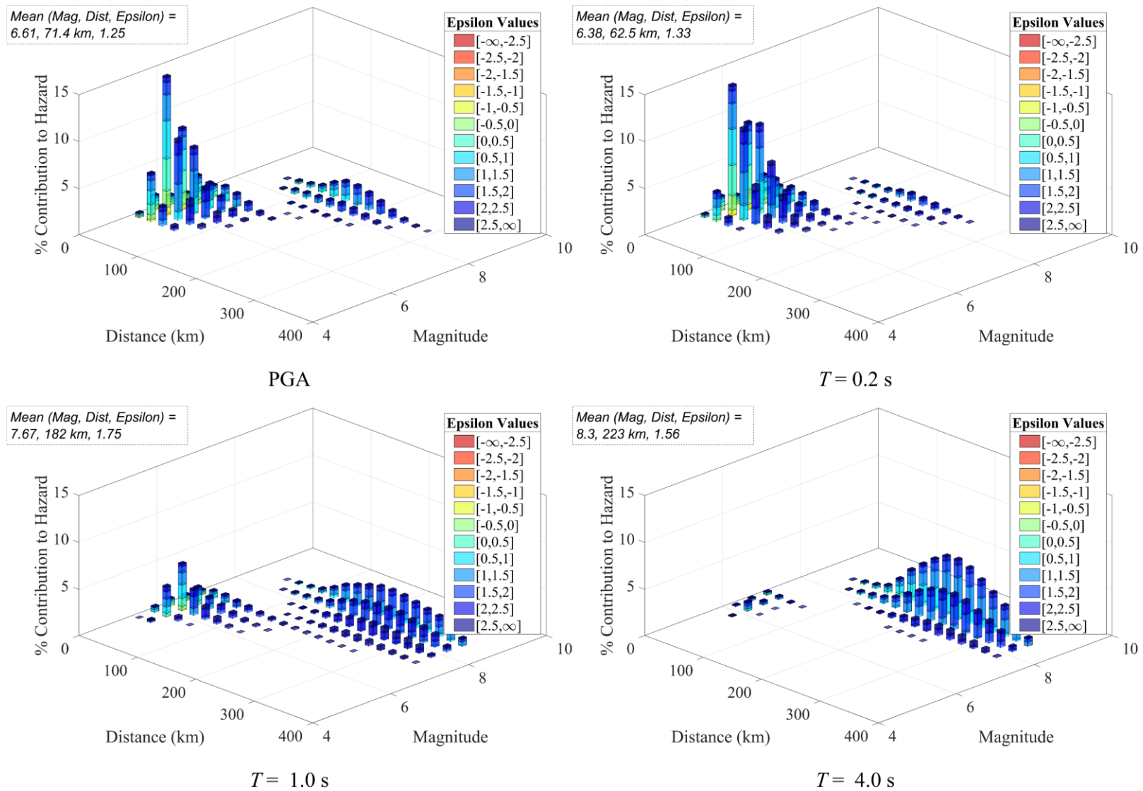
Fig. S10. Disaggregation of the hazard at the New Delhi site for 4500-year return period.
