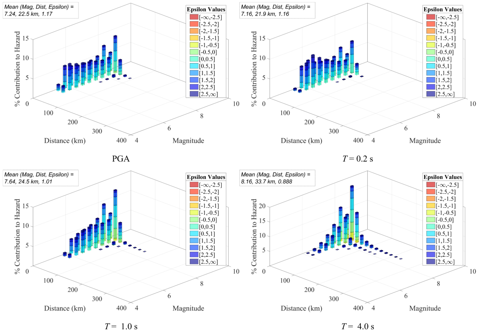
Fig. S4. Disaggregation of the hazard at the Dehradun site for 3500-year return period.
