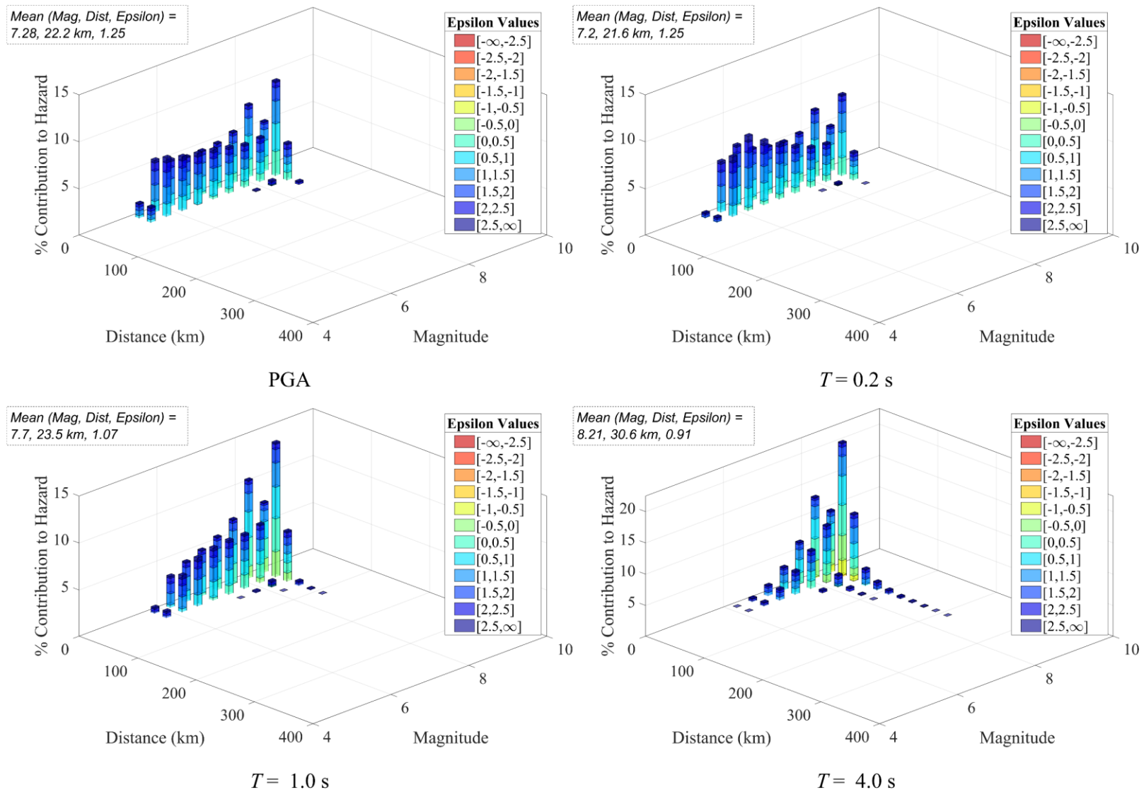
Fig. S5. Disaggregation of the hazard at the Dehradun site for 4500-year return period.
