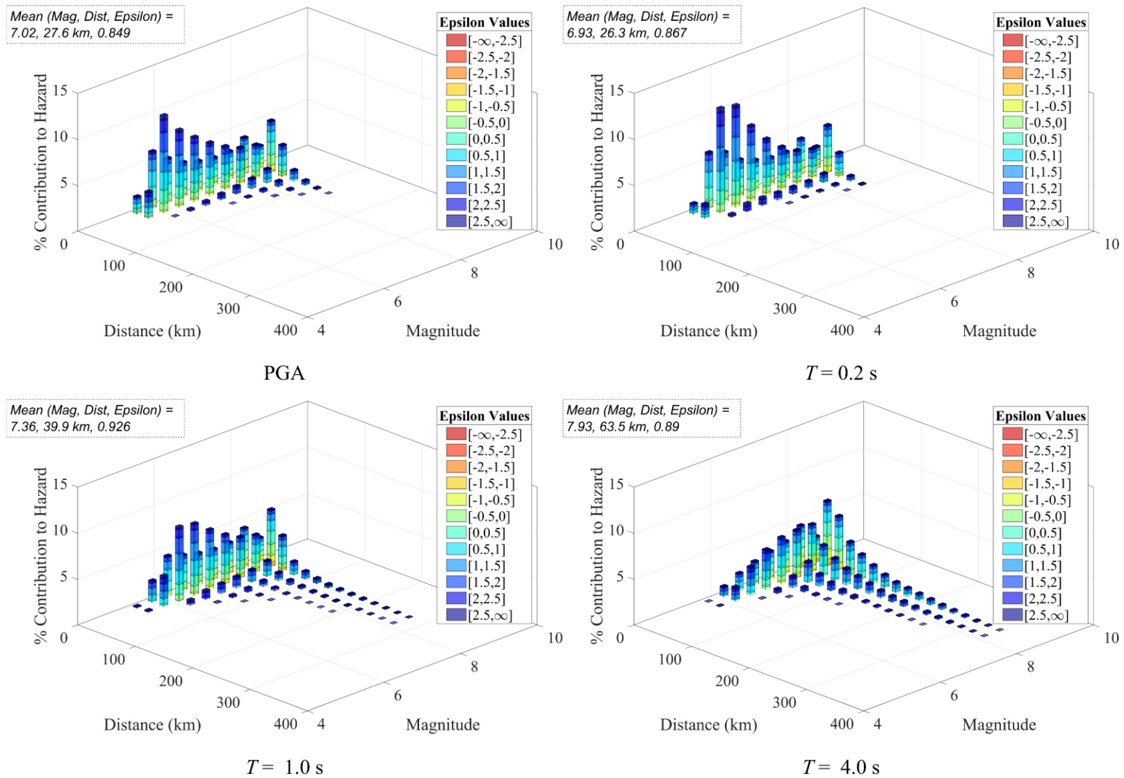
Fig. S1. Disaggregation of the hazard at the Dehradun site for 1000-year return period.
